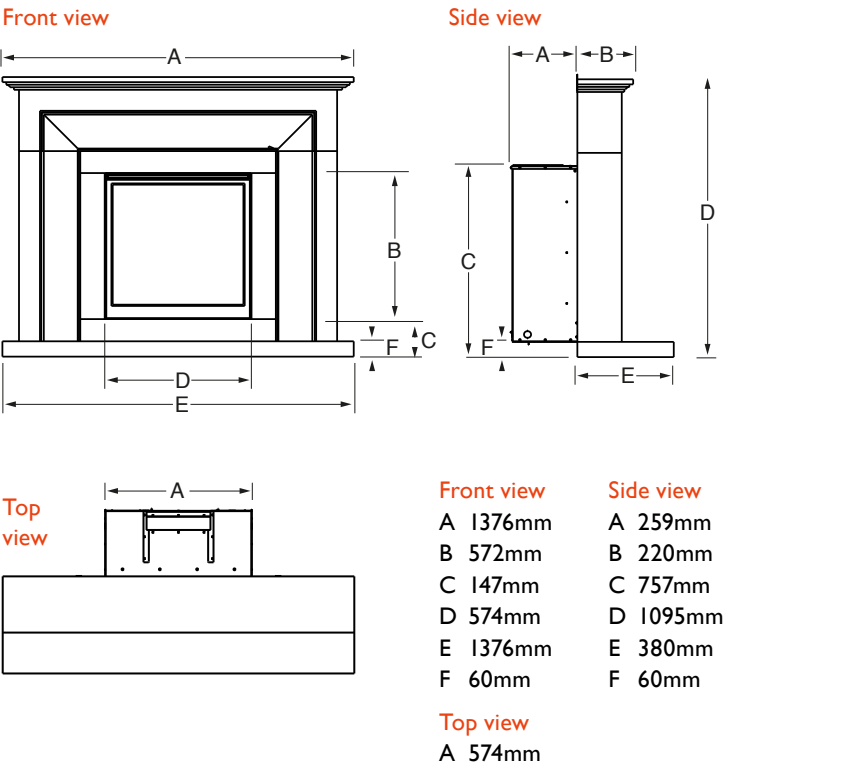
BOTICELLI CELENA SLIMLINE BALANCED FLUE
