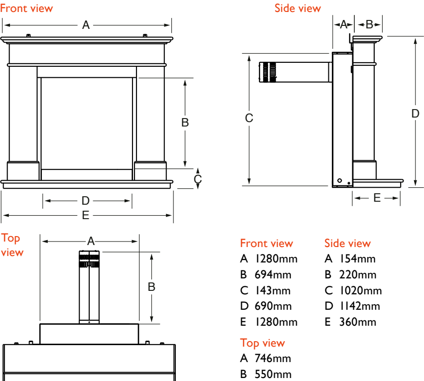
BOTICELLI ILLUMIA SLIMLINE BALANCED FLUE
